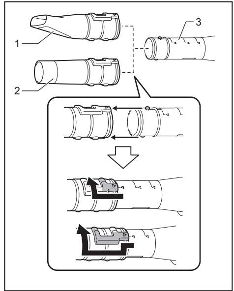
► 1. Flat nozzle 2. Extension nozzle 3. Blower pipe
